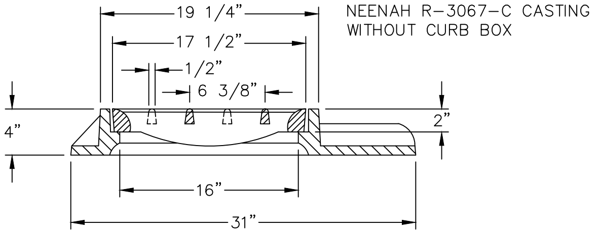
TYPE L GRATE
